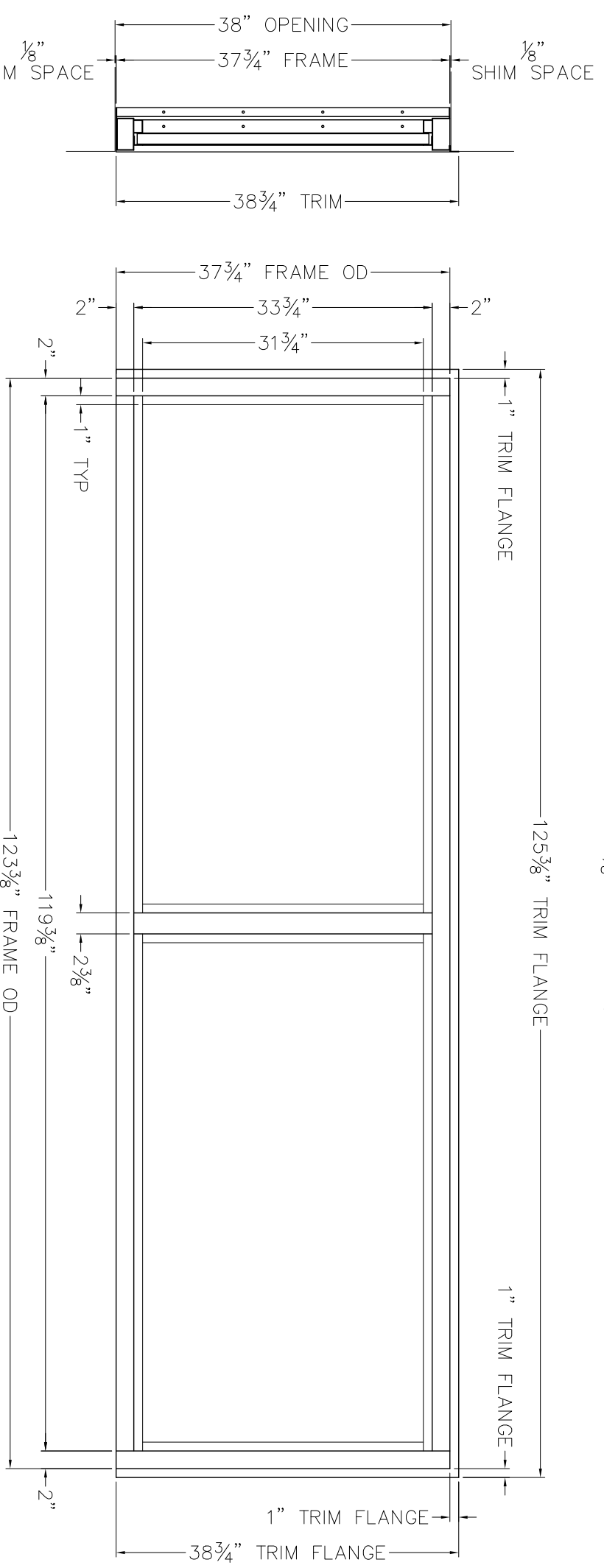
EXTERIOR ELEVATION (FRAME ONLY)
