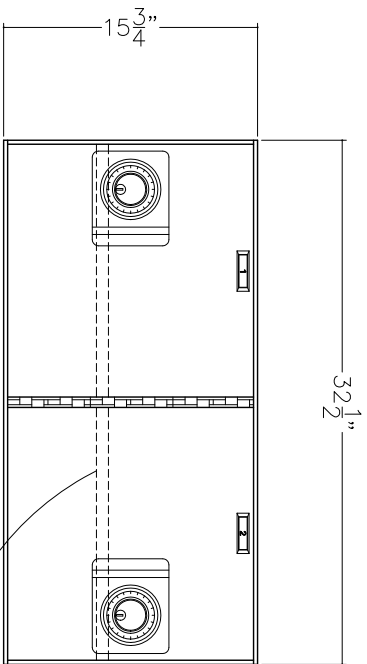
MODEL 560-2 (2) 15x16 OPENINGS
