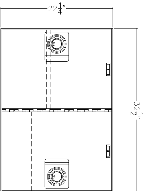
MODEL 563-2 (2) 22x16 OPENINGS
