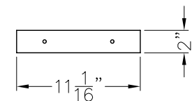
MODEL 521-9300 SPACER ASSEMBLY
