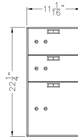
MODEL 521-3 (2) 5 x 10 OPENINGS (1) 10 x 10 OPENING
