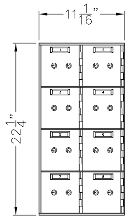
MODEL 521-8 (8) 5 x 5 OPENINGS
