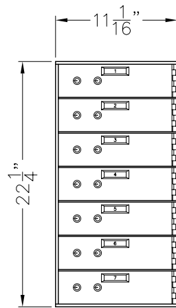
MODEL 521-7 (7) 3 x 10 OPENINGS
