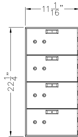
MODEL 521-4 (4) 5 x 10 OPENINGS
