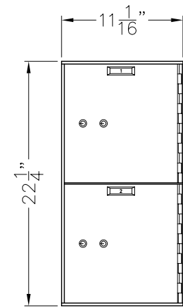
MODEL 521-2 (2) 10 x 10 OPENINGS
