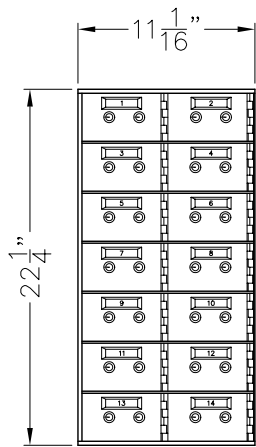
MODEL 521-14 (14) 3 x 5 OPENINGS
