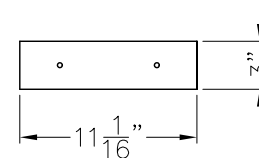
MODEL 521-9100 BASE ASSEMBLY
