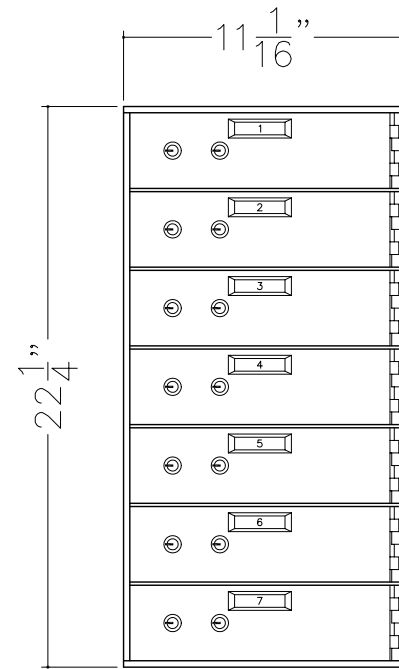
MODEL 521-7 (7) 3 x 10 OPENINGS
