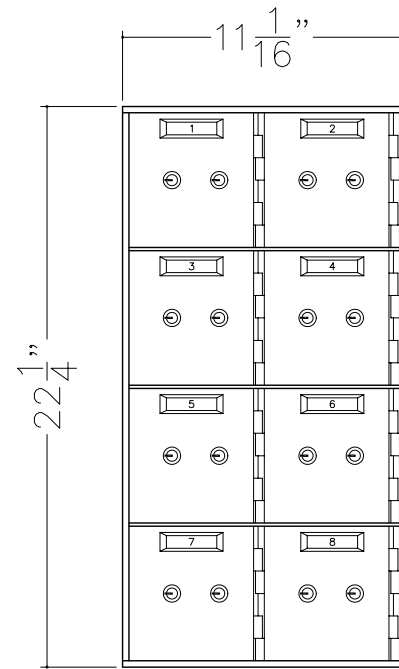
MODEL 521-8 (8) 5 x 5 OPENINGS
