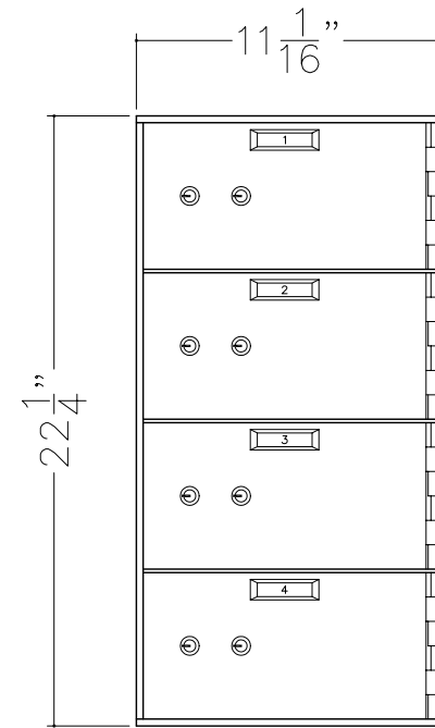
MODEL 521-4 (4) 5 x 10 OPENINGS
