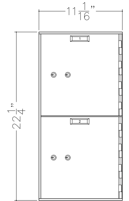
MODEL 521-2 (2) 10 x 10 OPENINGS
