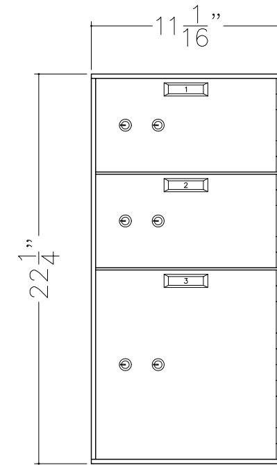
MODEL 521-3 (2) 5 x 10 OPENINGS (1) 10 x 10 OPENING
