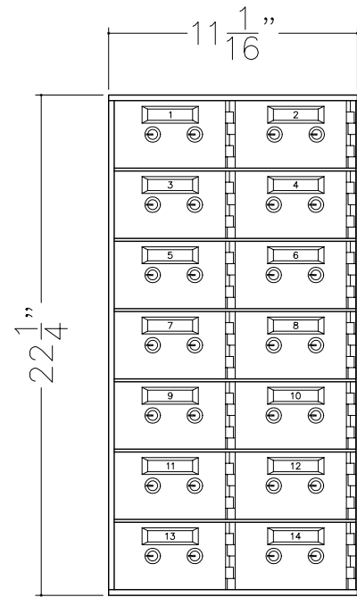
MODEL 521-14 (14) 3 x 5 OPENINGS
