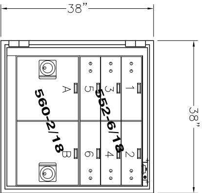
MODEL 981-1(6/2) (6) 5x16 TELLER LOCKERS (2) 15x16 CASH LOCKERS
