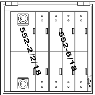
MODEL 981-1(8/2) (8) 5x16 TELLER LOCKERS (2) 10x16 CASH LOCKERS
