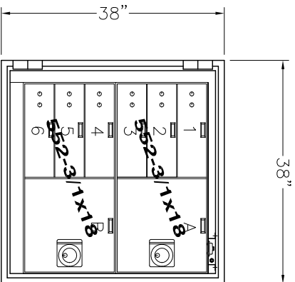
MODEL 981-1(6/2) A (6) 5x16 TELLER LOCKERS (2) 15x16 CASH LOCKERS
