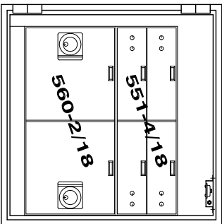
MODEL 981-1(4/2) (4) 5x16 TELLER LOCKERS (2) 15x16 CASH LOCKERS
