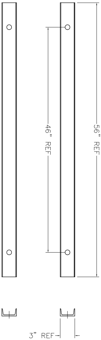
P/N 102-9939 (2 REQ'D)
